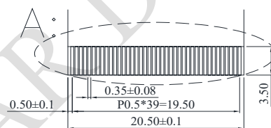
DETAIL A SCALE 3:1
