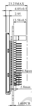
CON5
